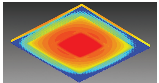
Figure 4: Temperature distribution on underside of a BGA package showing individual solder balls
