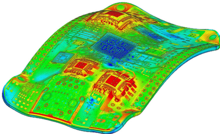
Figure 9: Von Mises stress caused by thermomechanical effects in a PCB with amplified out-of-plane displacement simulated in Simcenter FLOEFD.
