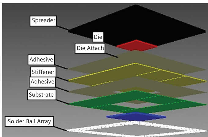
Figure 3: Thermally detailed thermal model of a chip package.
