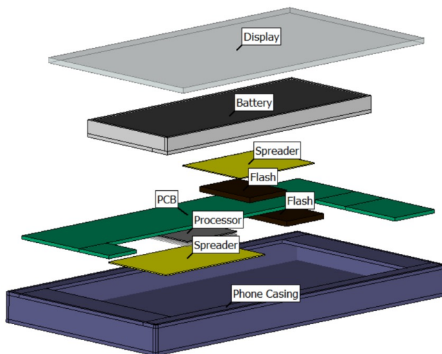
Figure 5: BCI-ROMs of key components in a mobile phone in PartQuest Explore
