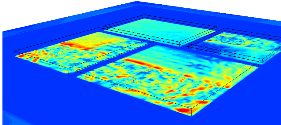
Figure 7: Detailed model of a multi-chip package with die power maps
