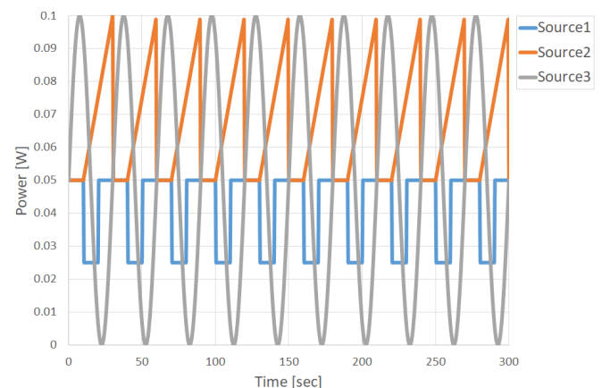
Figure 2: Example power vs. time profile
