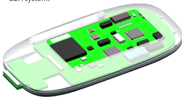
Figure 1: Thermal model of an insulin pump, with components modelled in different levels of detail.
